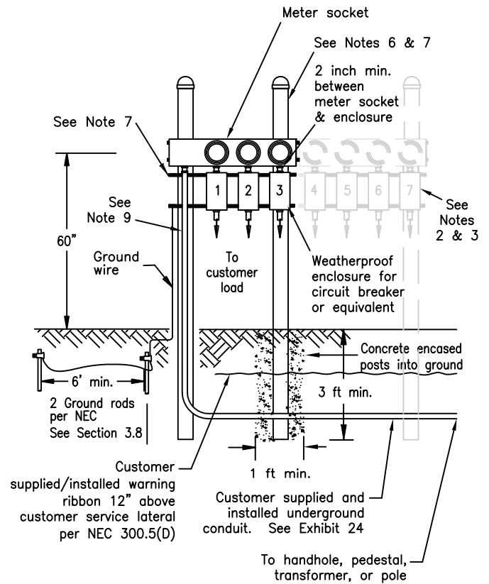
UNDERGROUND
