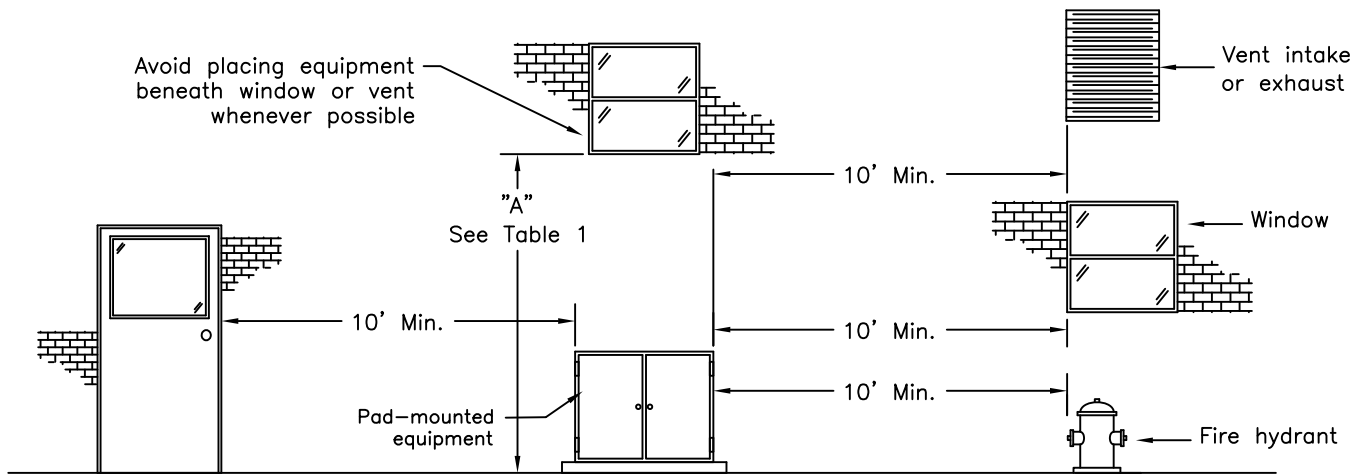
ELEVATION VIEW
